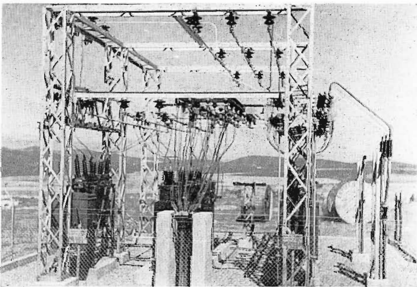
FIG. 5. Outdoor structure of the 35,000 volt sub-station, located at the transmitter site.
