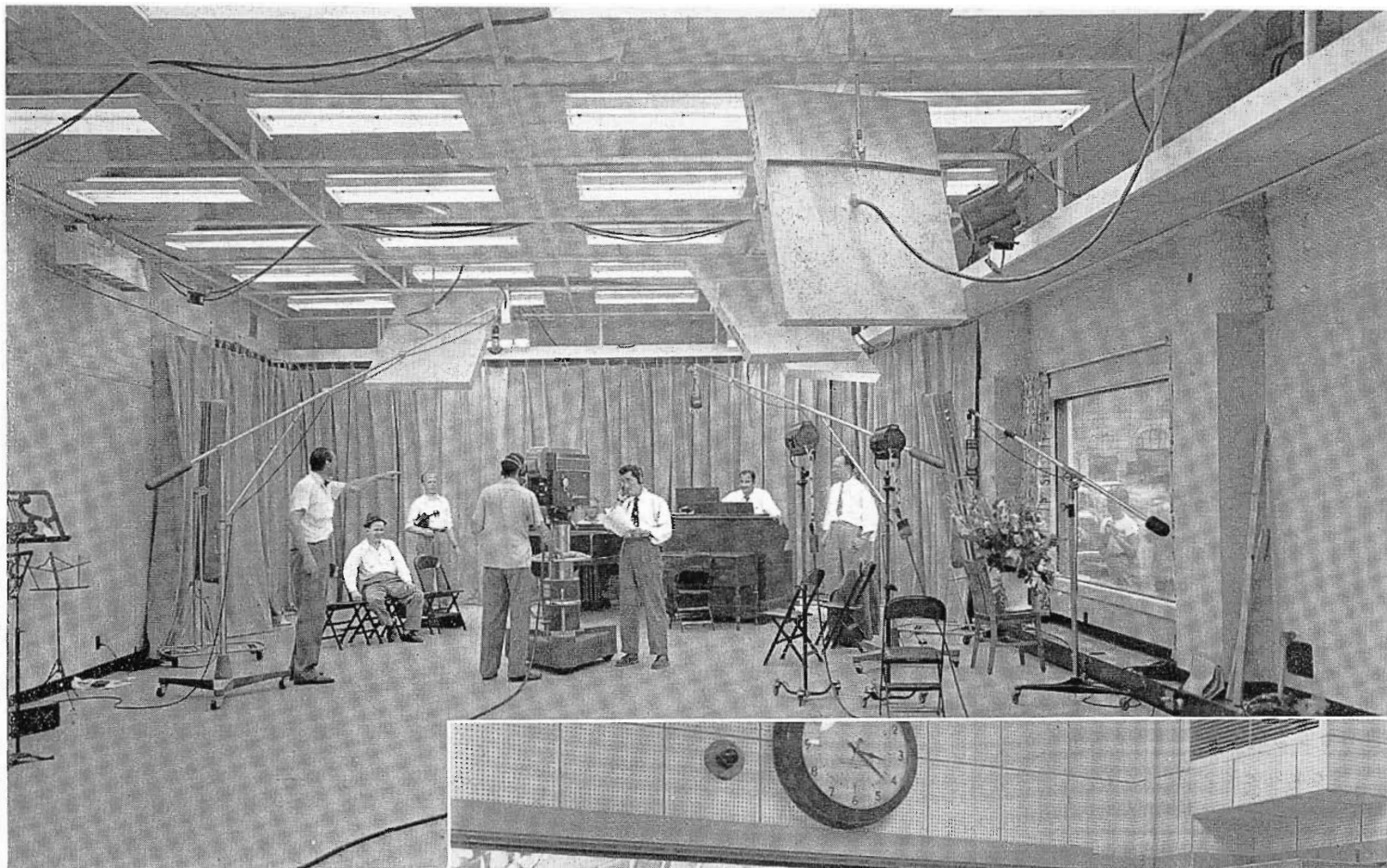
FIG. 6. The photo above shows the lighting facilities of WTCN's television studio which measures 30 by 50 feet. Garage-type doors, in rear, make it a simple matter to move scenery and equipment into the studio. Window at right, which is at street level, permits public to catch a glimpse of rehearsals.
