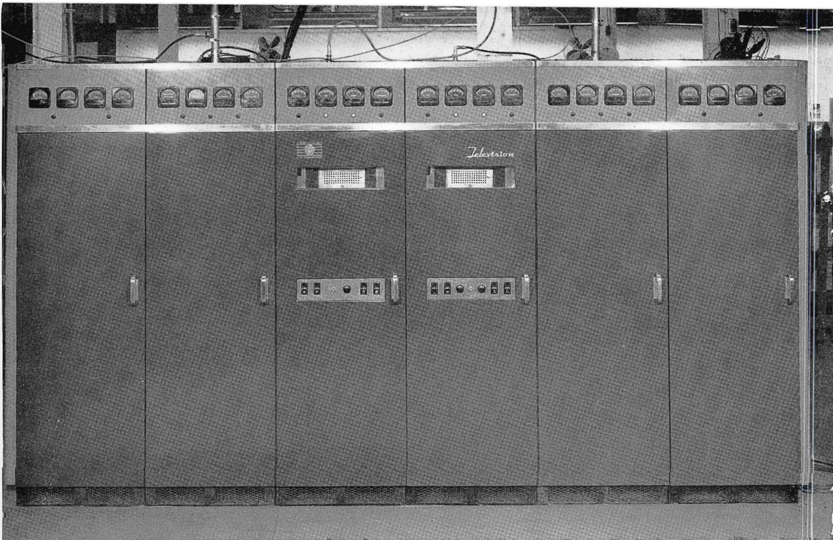
FIG. 1. THE RCA TTU-1A TELEVISION TRANSMITTER, designed for operation in the 530-890 mc band, is completely contained in six cabinet units which match, in appearance and size, the cabinets of RCA VHF transmitters and other RCA TV equipment. Overall dimensions are 150" long, 84" high and 31" deep. The transmitter, which provides an output of 1 kw at low end of the band (slightly less at high end), is completely air-cooled.
