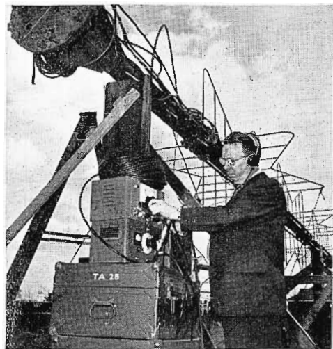
Ground-checking a 3-bay TV Super-Turnstile
