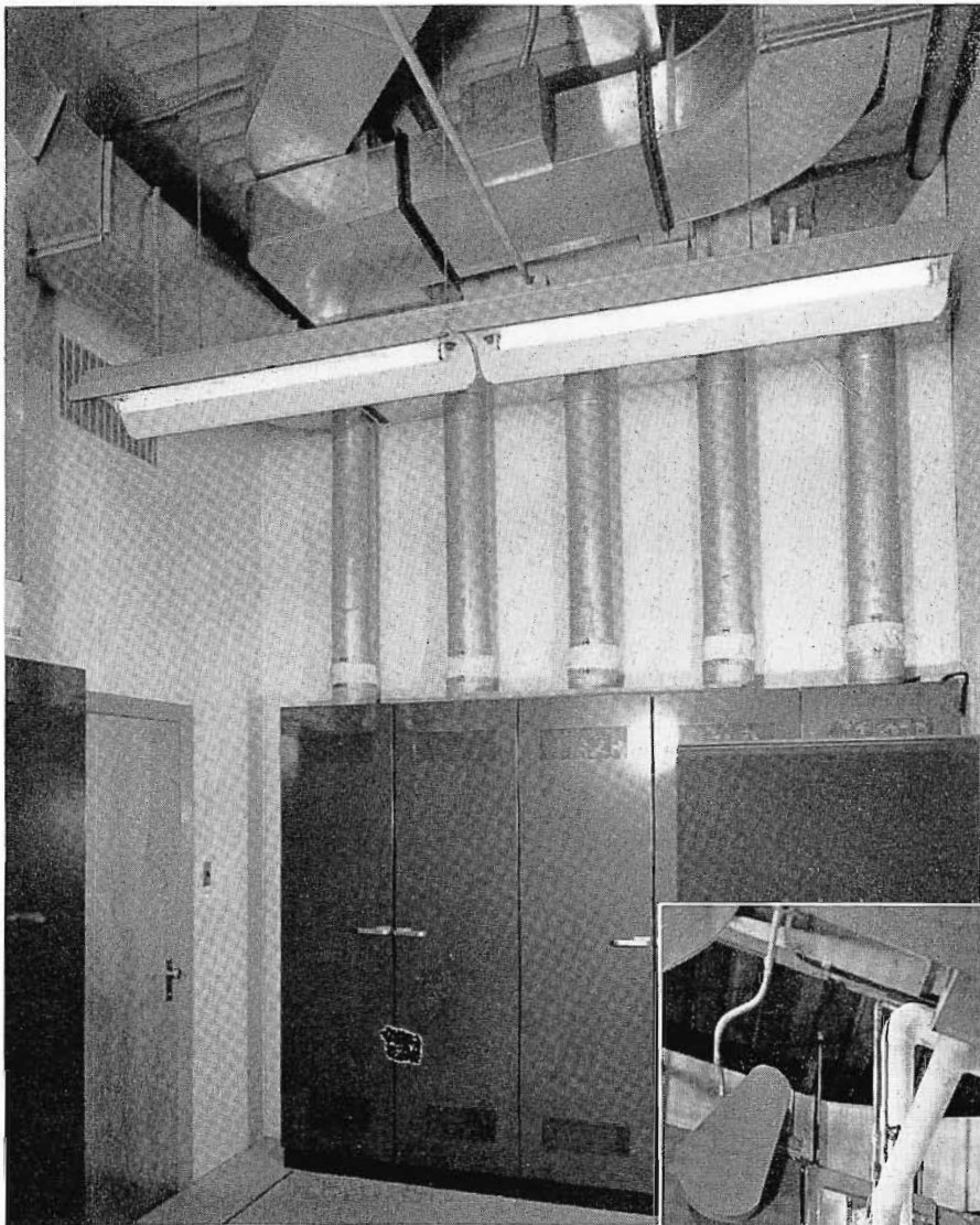
FIG. 16 (left). This is a view in the "test and storage" room adjacent to the studio control room. The back of the video cabinet racks (which face into the control room) is seen here. Ducts are used to exhaust heat from the equipment racks directly to the outside during the summer time, or for recirculating it to the station's heating system in cold weather.
