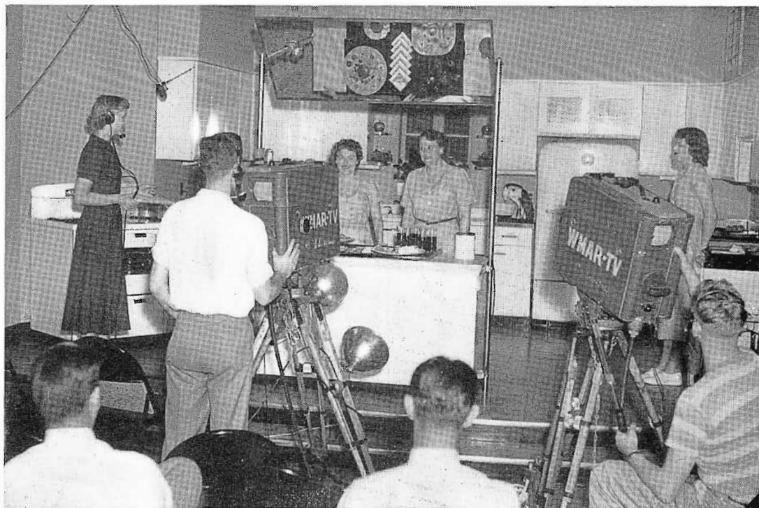
FIG. 4. Field cameras are used to telecast remote cooking demonstration. Note overhead mirror technique used in displaying dishes described.
