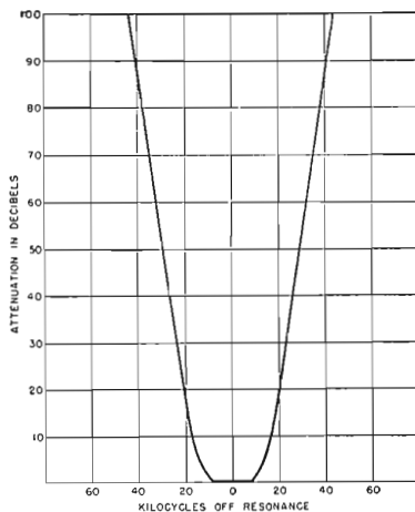
"CANYON-CURVE" SELECTIVITY
