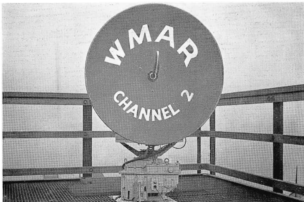
FIG. 14. Standard microwave relay dish, mounted on a Navy surplus radar base, permits remote control of horizontal and vertical positions.
