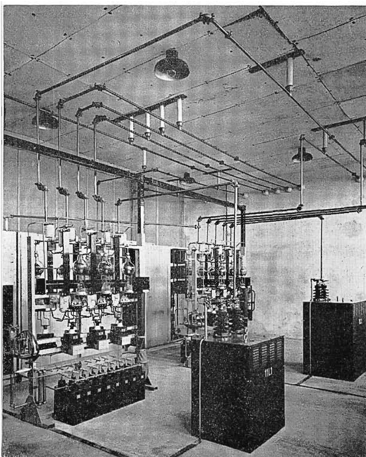
FIG. 6. Shown below are the medium and high voltage rectifier units.
