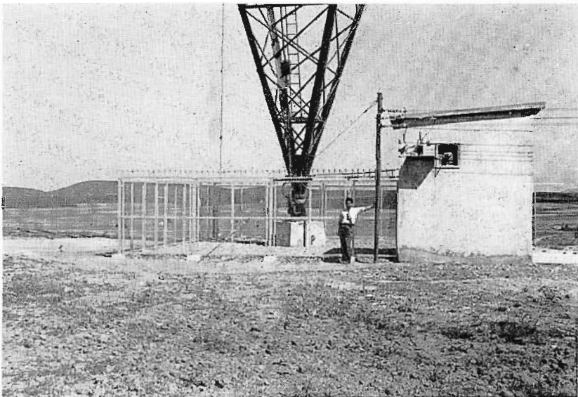
FIG. 4. The antenna tuning house and base of the 725-foot vertical radiator.
