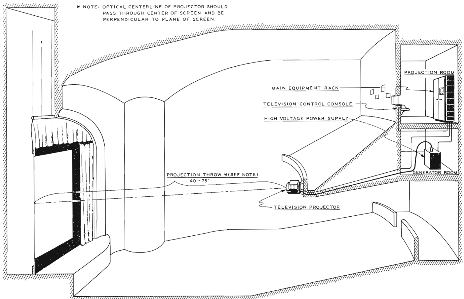
TYPICAL INSTALLATION OF INSTANTANEOUS PROJECTION SYSTEM
