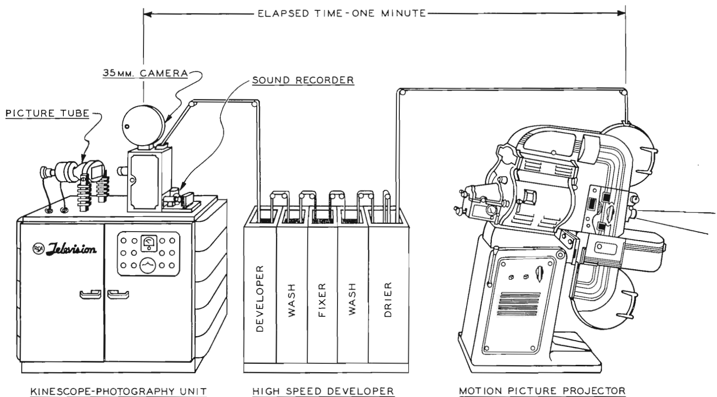
RCA "INTERMEDIATE FILM" THEATRE TELEVISION SYSTEM
