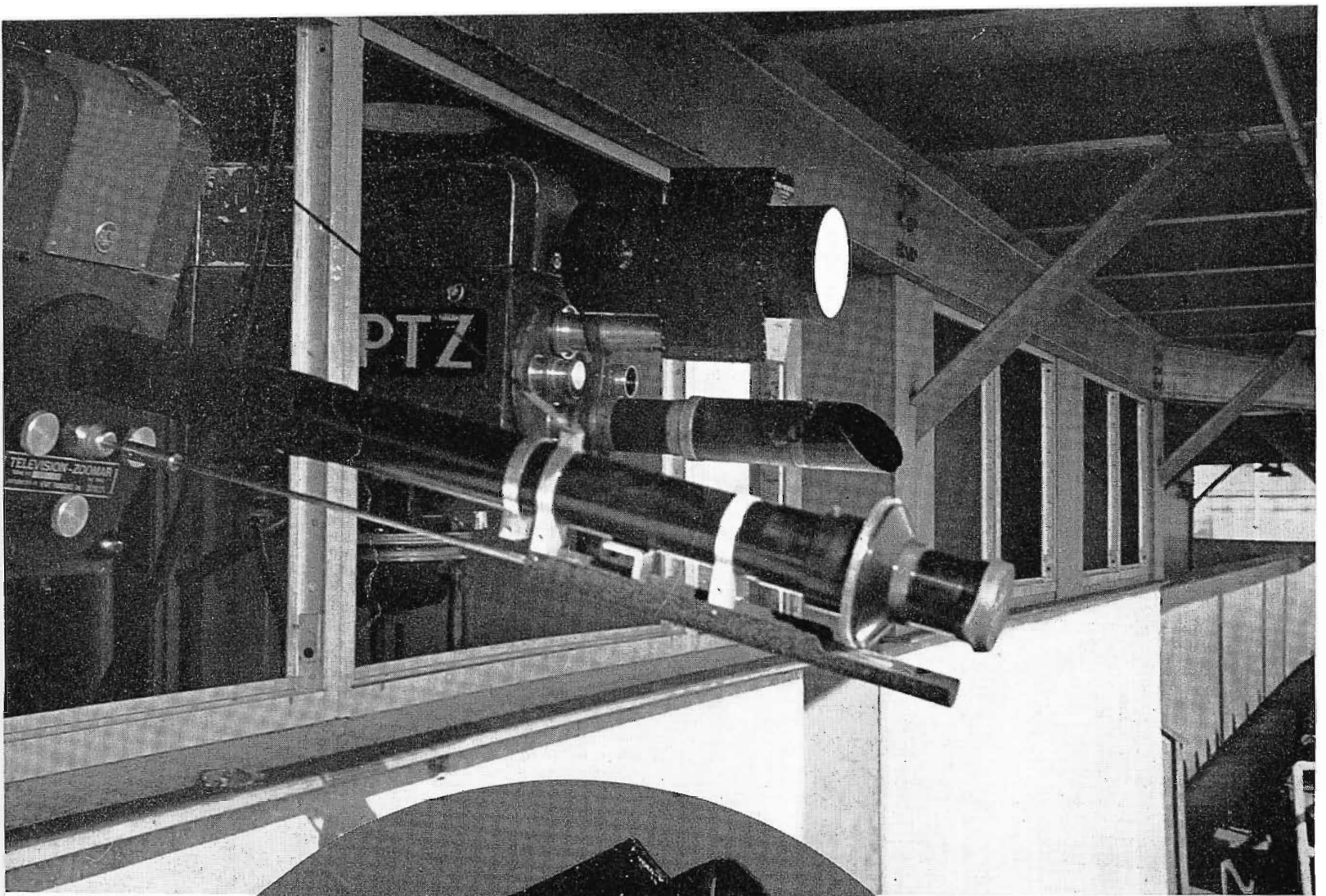
FIG. 1 (above). WPTZ's No. 1 camera (with Zoomar) and No. 2 camera (with Reflector) in press box at Municipal Stadium. Although nearly 300 feet from the field the Reflector's 40-inch focal length made possible closeups of action during the game.
