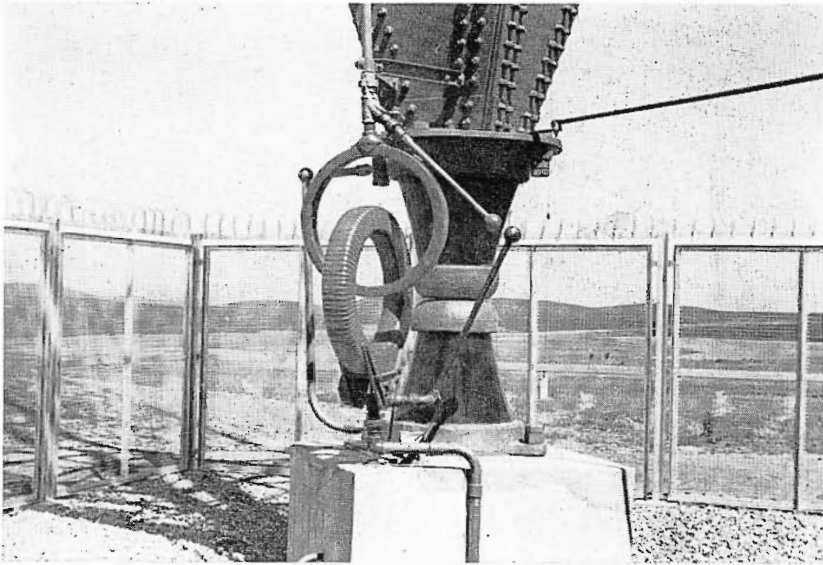
FIG. 3. The antenna tower base, showing toroidal-type lighting transformer and ball gaps.
