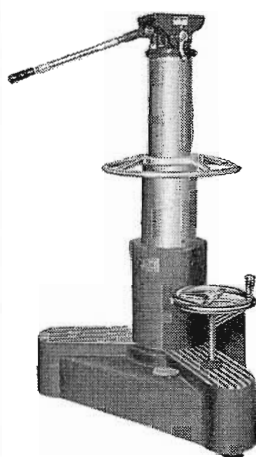
STUDIO CAMERA PEDESTAL, TD-1A —Television's favorite pedestal for studio and other indoor operations. Moves freely, quietly. Crank handle raises and lowers camera to any height between 40 inches and five feet above the floor. Moves in any direction—or about a point. Panning and tilting provided by Friction Head MI-26205.
