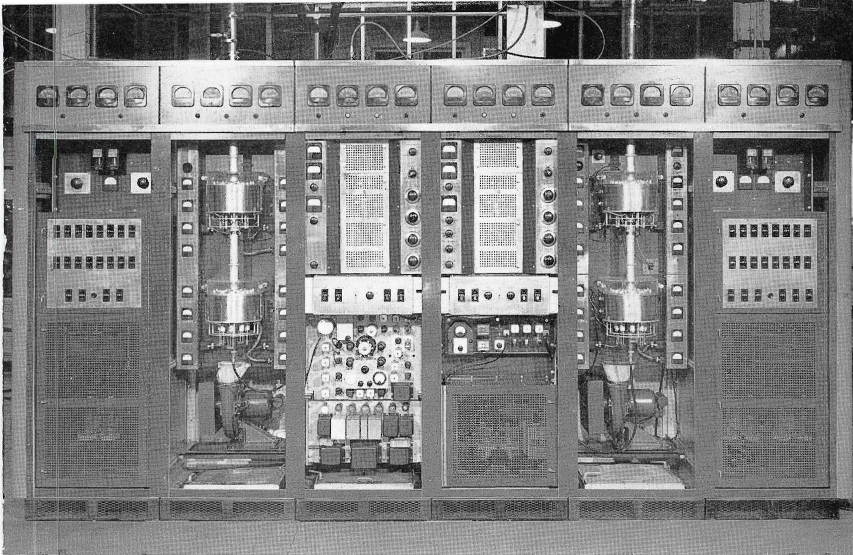
FIG. 2. INTERIOR OF THE TTU-1A TRANSMITTER with doors removed to show construction. The cabinet units, from left to right, contain: (1) the aural section power supplies and control circuits, (2) the aural section tripler and power amplifier stages, (3) the aural driver section, (4) the visual driver section, (5) the visual section tripler and power amplifier stages, and (6) the visual section power supplies and control circuits.
