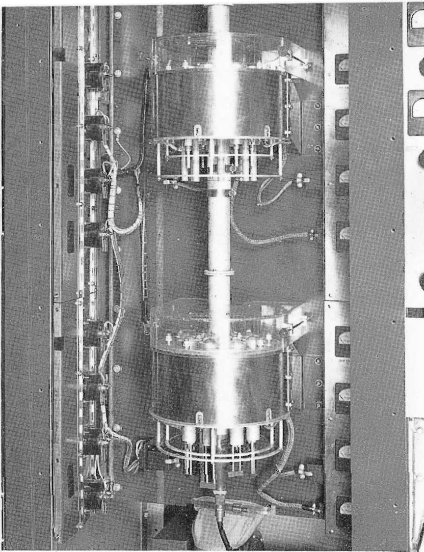
FIG. 5. RING AMPLIFIERS used in the UHF section of the TTU-1A Transmitter. The tripler and P.A. stage, shown above, each consist of eight 4X150A's mounted in a circle in a single cavity and connected in parallel. (A view looking down on one of these cavities is shown on the cover of this issue). Each cavity consists of three concentric cylinders (of which only the outside one is visible). The cylinders are capped by three flat circular plates which form the anode, screen and grid plates. These plates provide a base on which the tubes are mounted. D-C cathode connections are brought out separately so that the tubes may be metered individually. This facilitates proper distribution of load between tubes, and quick detection of tube failures. A plastic shield over the top of the assembly aids in forced air cooling of the tubes and provides a safety cover. The whole cavity assembly is a plug-in unit so that a spare may be easily inserted.
