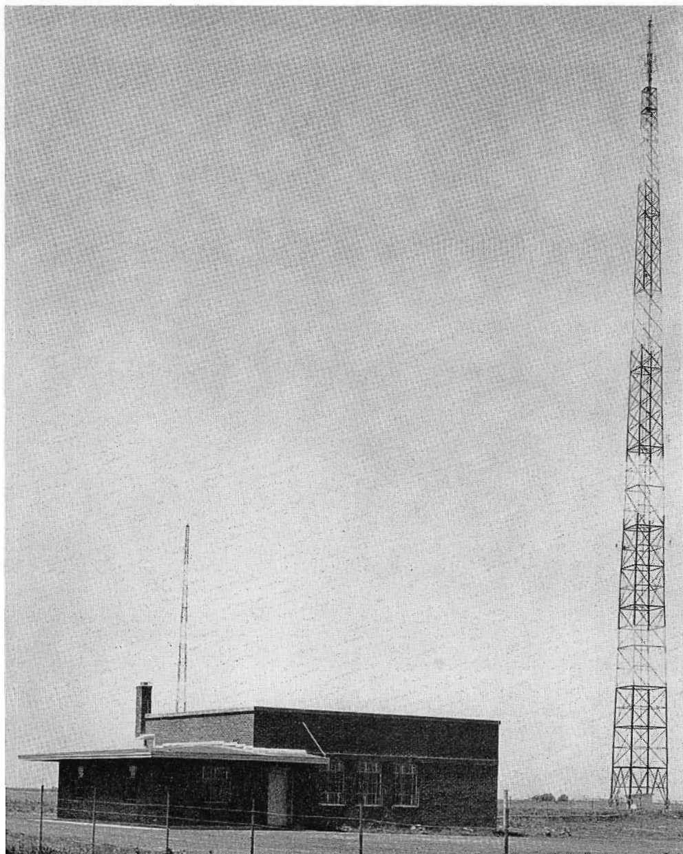
FIG. 5. KSEI employs a two element directional antenna system. The 255-foot tower at left is used for nighttime AM transmission; the one at the right for AM daytime. An RCA two-element Superturndale FM antenna is mounted atop the AM tower at right.
