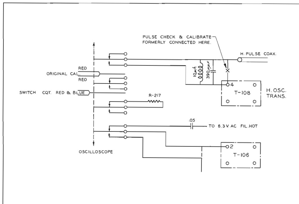
FIG. 1. Circuit changes in TM-5A Monitor for "Pulse Cross" measurements.
