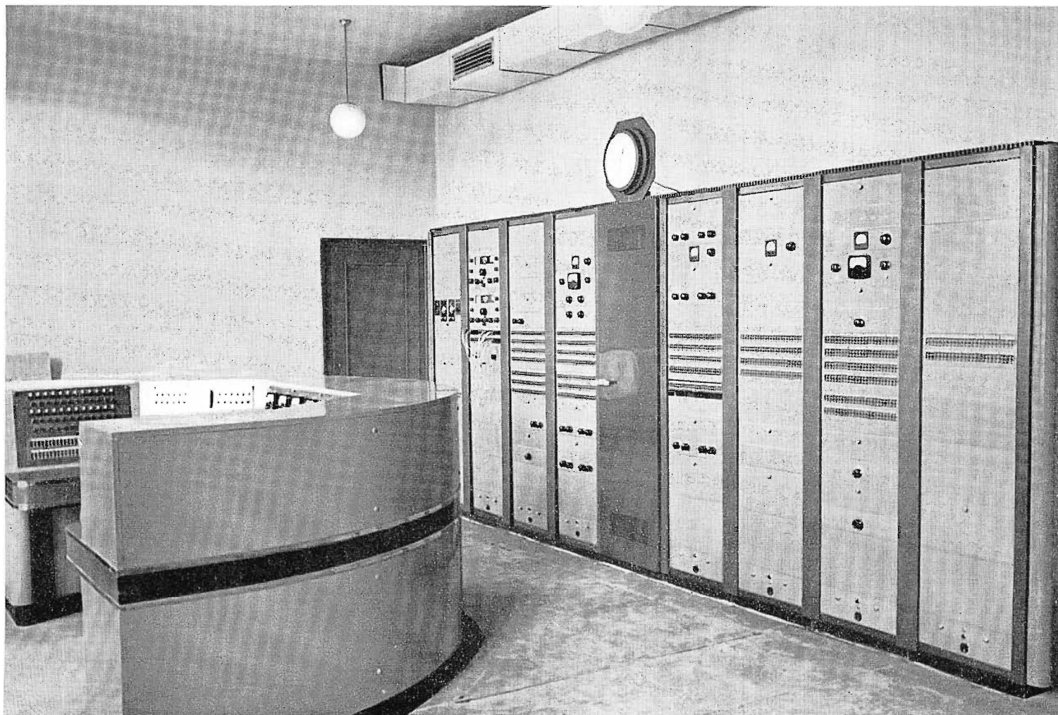
FIG. 11. Another view of the equipment racks and control desk in the studio master control room.
