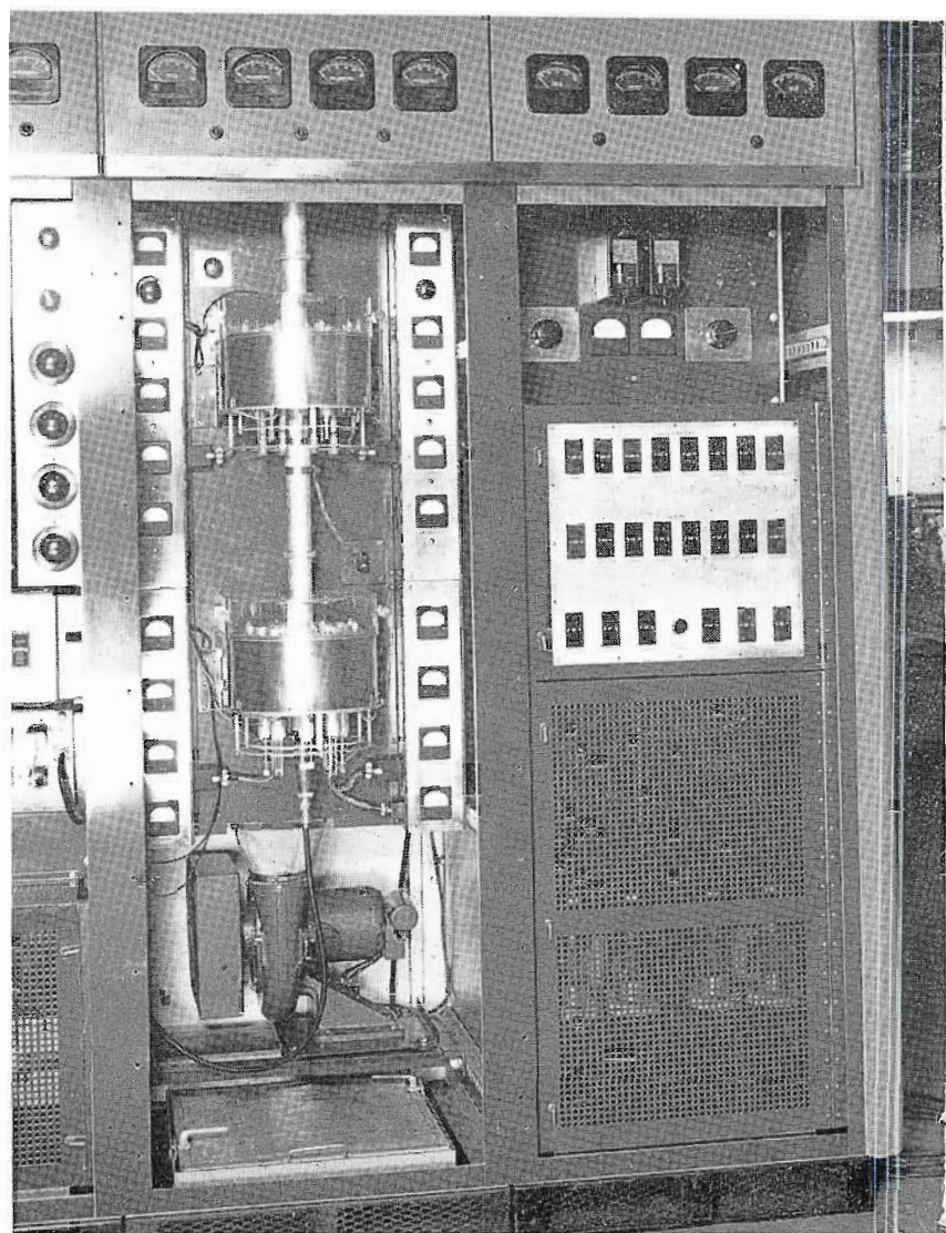
FIG. 4. VISUAL AMPLIFIER SECTION of the transmitter. The r-f and modulator circuits are in the left-hand cabinet, the power supplies and controls are in the right-hand cabinet. The r-f portion consists of two stages, a tripler and a power amplifier. The tripler stage consists of eight 4X150A's connected in parallel and mounted in a single ring-type cavity. This is the drum-like unit in the lower part of the cabinet. R-F power is fed to this unit, from the driver, by the flexible coax at the bottom. A short length of concentric line leads from the top of the tripler cavity to the power amplifier cavity, which is the similar appearing drum directly above. The power amplifier employs eight 4X150A's mounted in a ring-type cavity very similar to that of the tripler stage. The grids of the P.A. tubes are modulated by a video amplifier (made up of eight 6L6's) which is driven by the three-stage video amplifier in the driver unit.
