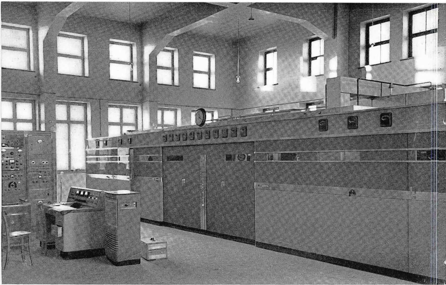
FIG. 1. The RCA Type BTA-150A Transmitter installed at Radio Istanbul, Turkey. The transmitter control console and test and measuring equipment racks are shown at left.
