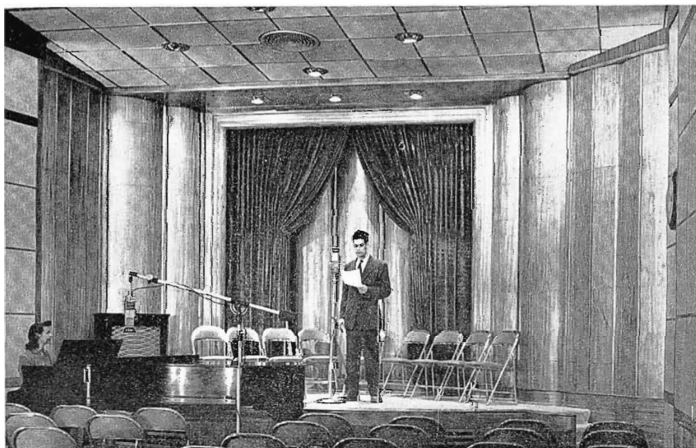
FIG. 7. Studio A, which shares a control room with Studio B, seats about 150 people. Backstage curtains offer a degree of acoustic control by exposing or covering polycylindrical diffusers.
