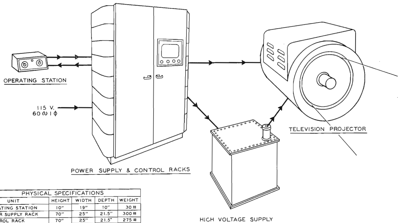
RCA INSTANTANEOUS "PROJECTION" THEATRE TELEVISION SYSTEM
