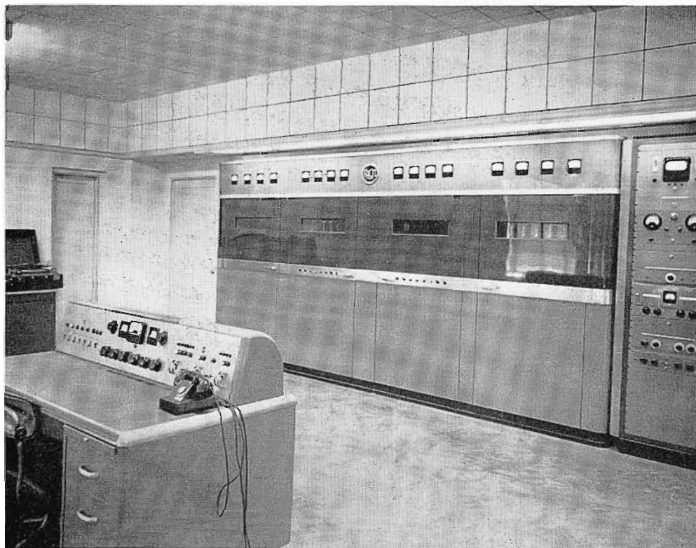
FIG. 1. Photo above shows the transmitter control room of Station KSEI. Recessed fluorescent lighting is used to illuminate the meters of the RCA 5 KW AM transmitter and the speech input racks. The transmitter control console is shown at left.
