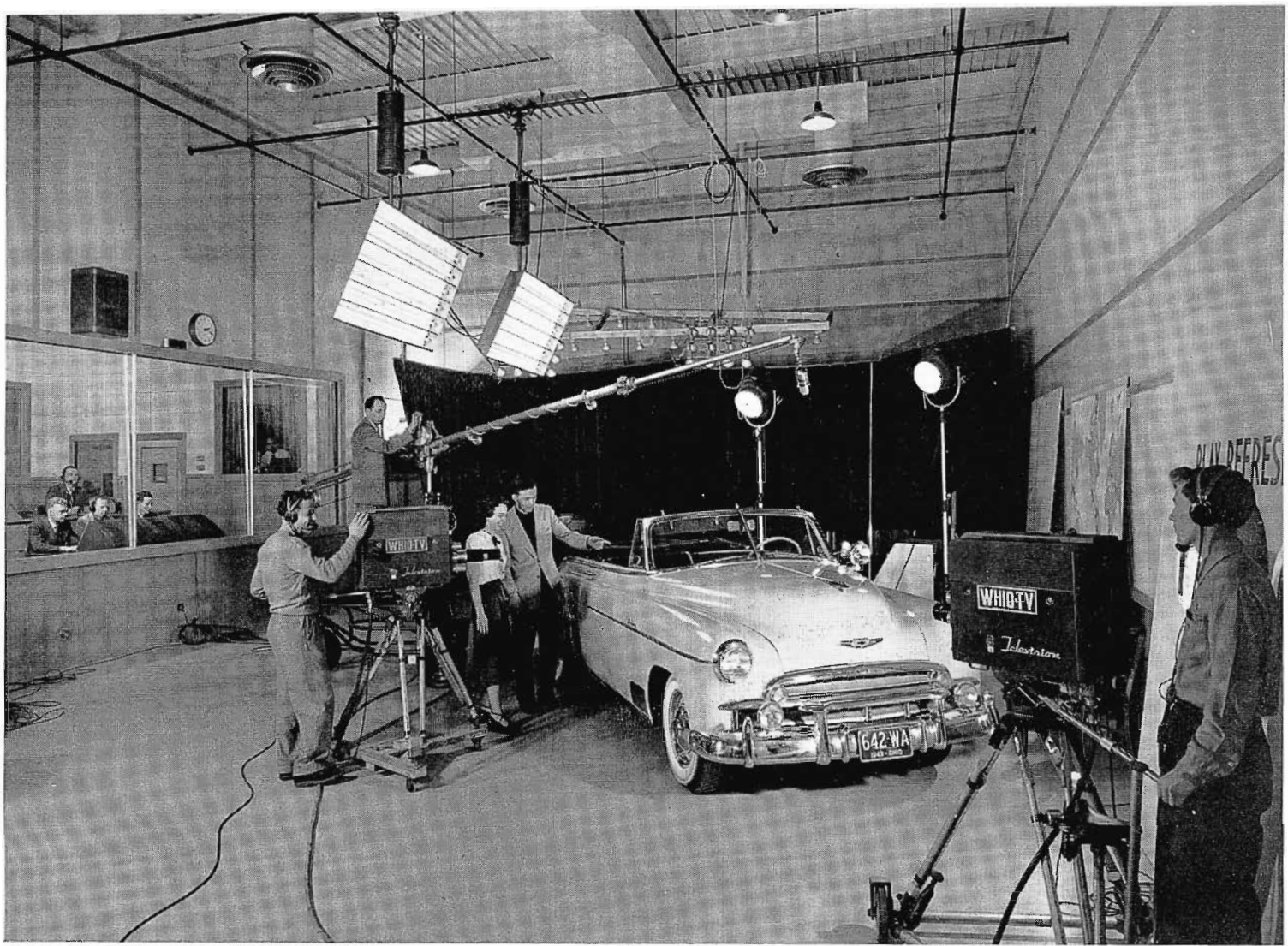
FIG. 11. WHIO-TV's ground level studio, with garage-type doors, allows cars and trucks to be driven directly onto the studio floor—either for bringing in display material or for actual telecasting, as shown here.
