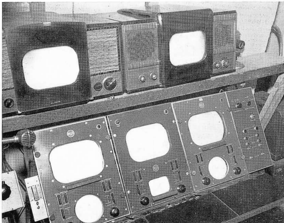
FIG. 9. Bank of monitors in TV film room include two camera control monitors (lower left), an outgoing picture monitor, and station-built dissolve panel. TV receivers, on shelf above, are used as closed circuit and "off-the-air" monitors.
